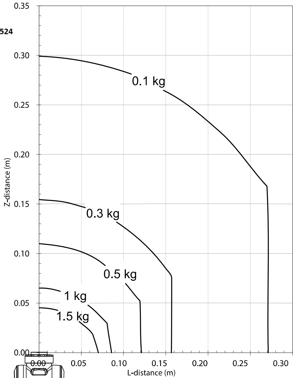
Diagrams of IRB 1010-1.5/0.37
